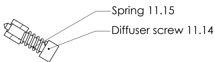
CROSS SECTION A-A
